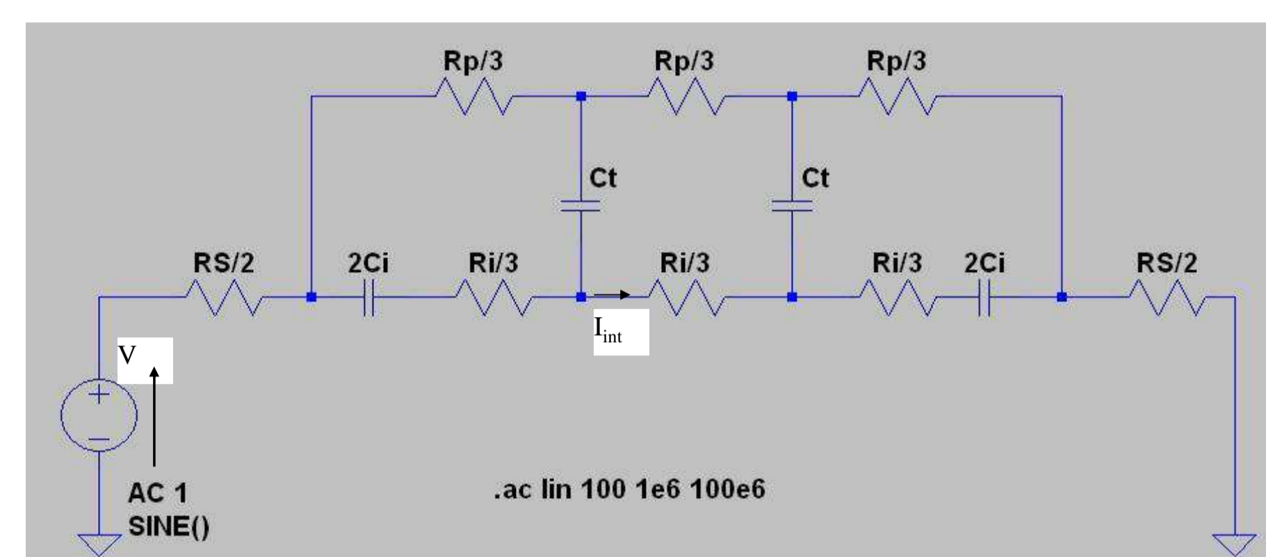
Figure 3. Equivalent circuit of the box, longitudinal Excitation
