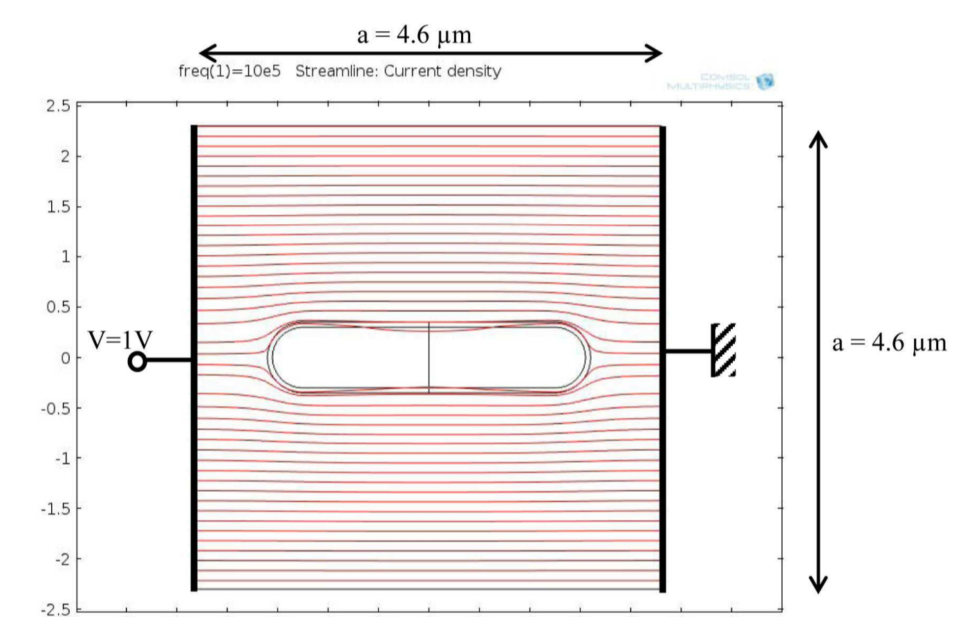
Figure 4. Current streamlines, longitudinal excitation @ f = 1MHz
