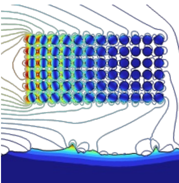
Figure 4 : Thumbnail - Effect of surface roughness on eddy current probe response
