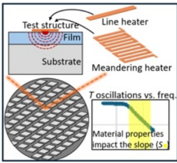
Figure 4 : The test insertions 3 \omega -methodology to monitor wafers quality after the front-end in production flow for thermal flow sensors.
