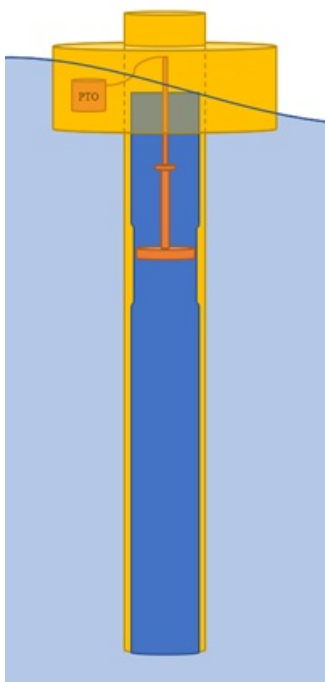
Figure 1 : Schematic view of the WaveEL buoy.
