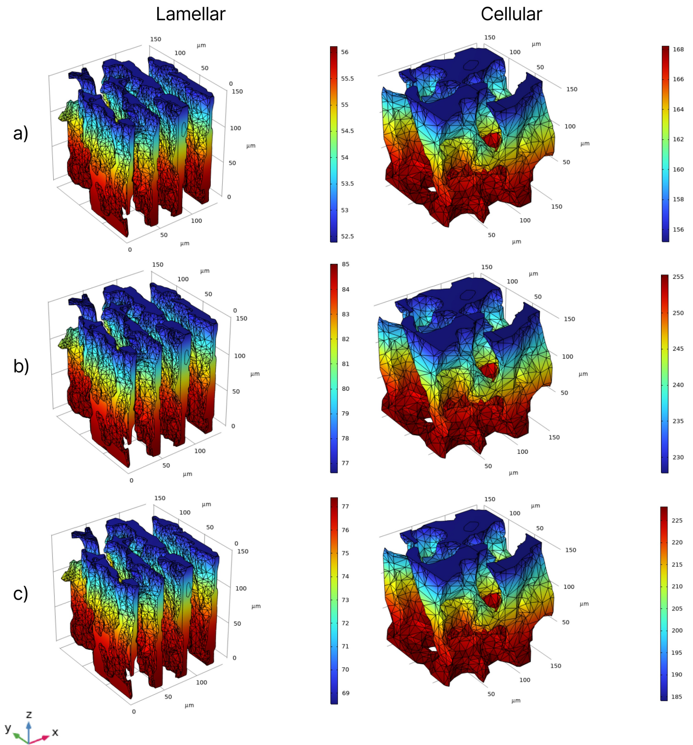
Figure 3 : Local current densities of cellular and lamellar microstructures under discharge current densities of a) 50, b) 75, and c) 100 A/m 2 .
