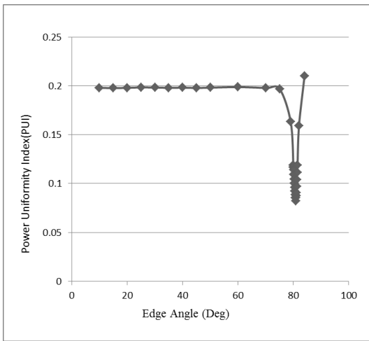
Figure 2 Power uniformity index as a function of the edge angle of the applicator.
