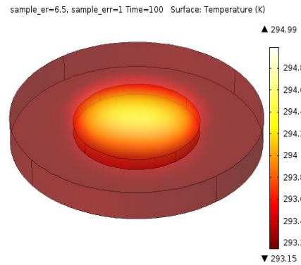
Figure 3. Typical coupled electro thermal results and temperature distribution for Dielectric constant of 6.5 and loss factor 1
