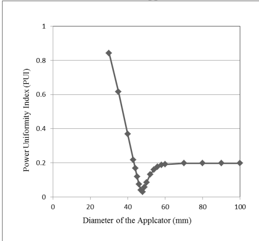
Figure 1. Power uniformity index as a function of the diameter of the applicator.
