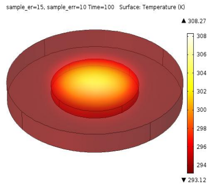
Figure 4. Typical coupled electro thermal results and temperature distribution for Dielectric constant of 15 and loss factor 10
